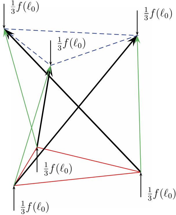
Figure 3.30: Minimal regular tensegrity prism under compressive load
