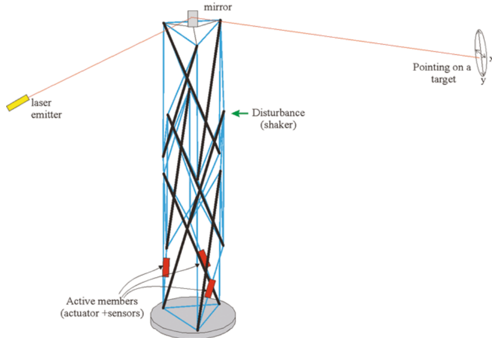
Figure 1.41: The Experimental setup for vibration control of a tensegrity column
