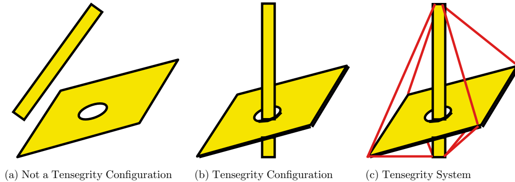
Figure 1.1: Two-body configurations
