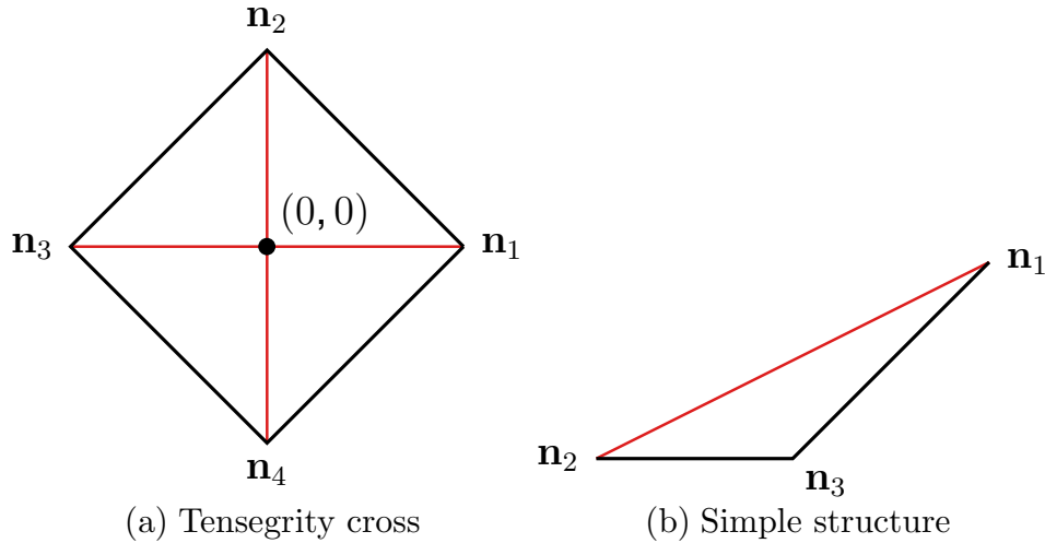
Figure 2.4: Dual structures
