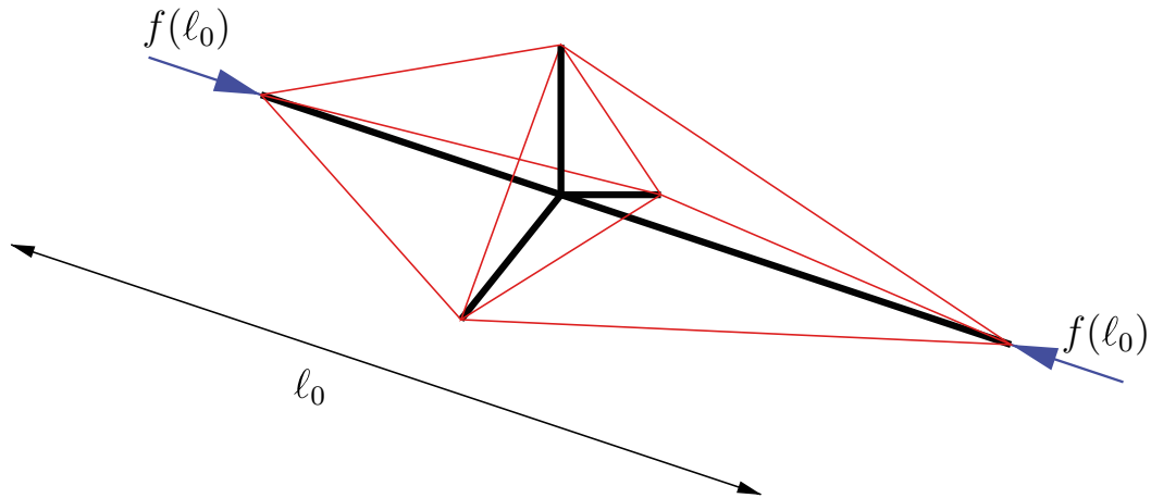
Figure 3.15: Three-dimensional T-Bar system
