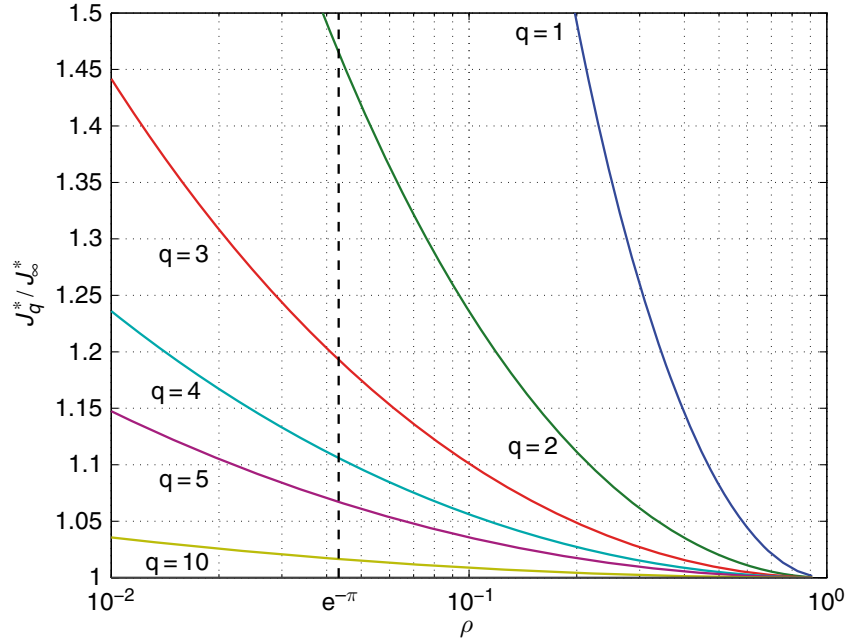
Figure 4.12: The relative optimal discrete cost J_q^*/J_\infty^* ; material overlap occurs for \rho \leq e^{-\pi}
