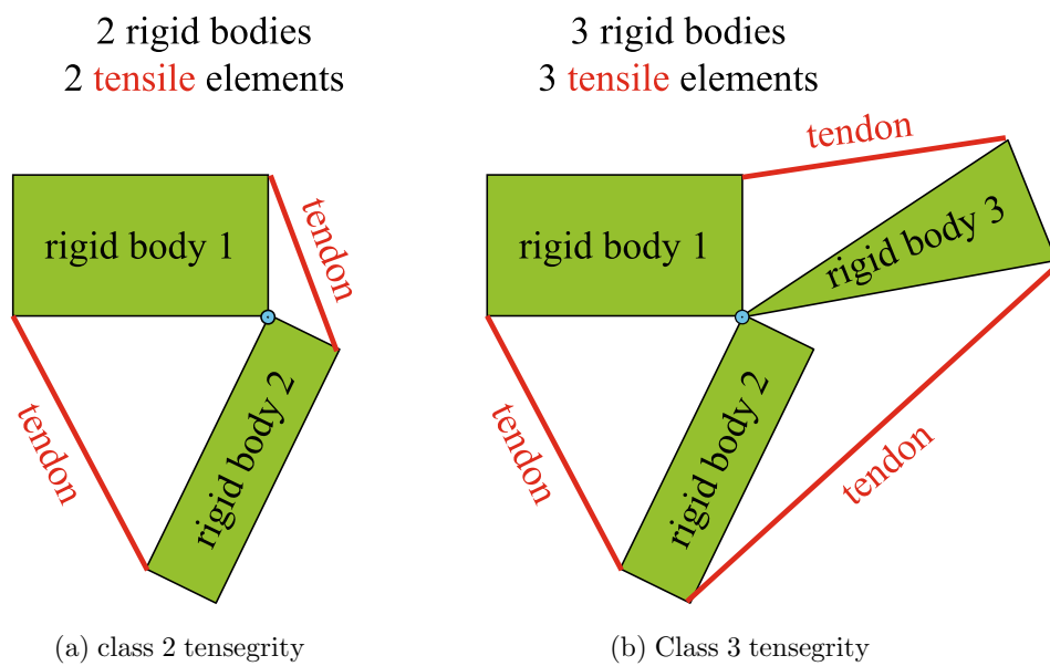
Figure 1.5: A class 2 and a class 3 tensegrity system
