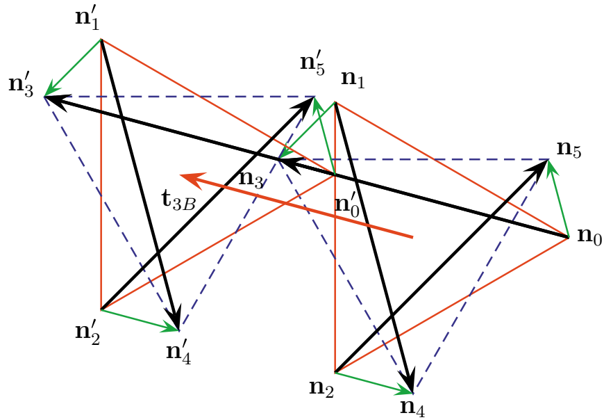
Figure 3.37: Three-bar plate connection – topology B – top view
