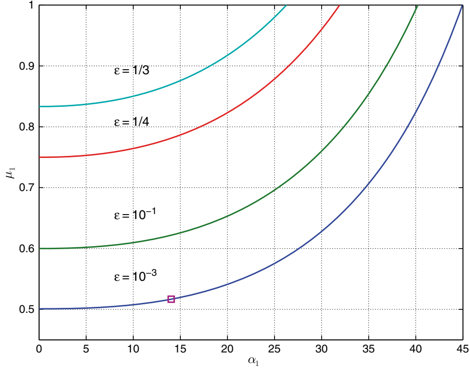
Figure 3.6: T-Bar unit: \mu_1 versus \alpha_1 , from (3.10)
