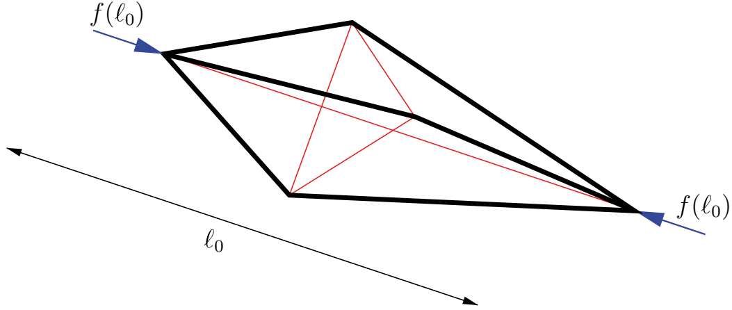
Figure 3.22: A three-dimensional D-Bar unit
