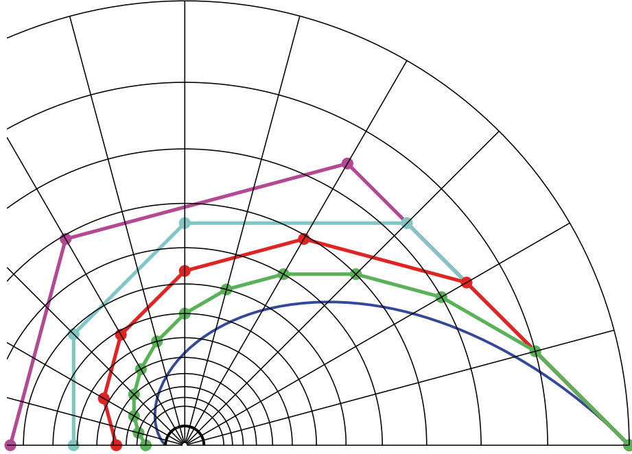
Figure 4.11: Discrete Michell Spirals of order 3, 4, 6, 12, and \infty (continuous) ( q\phi = \pi , \beta = \pi/4 )
