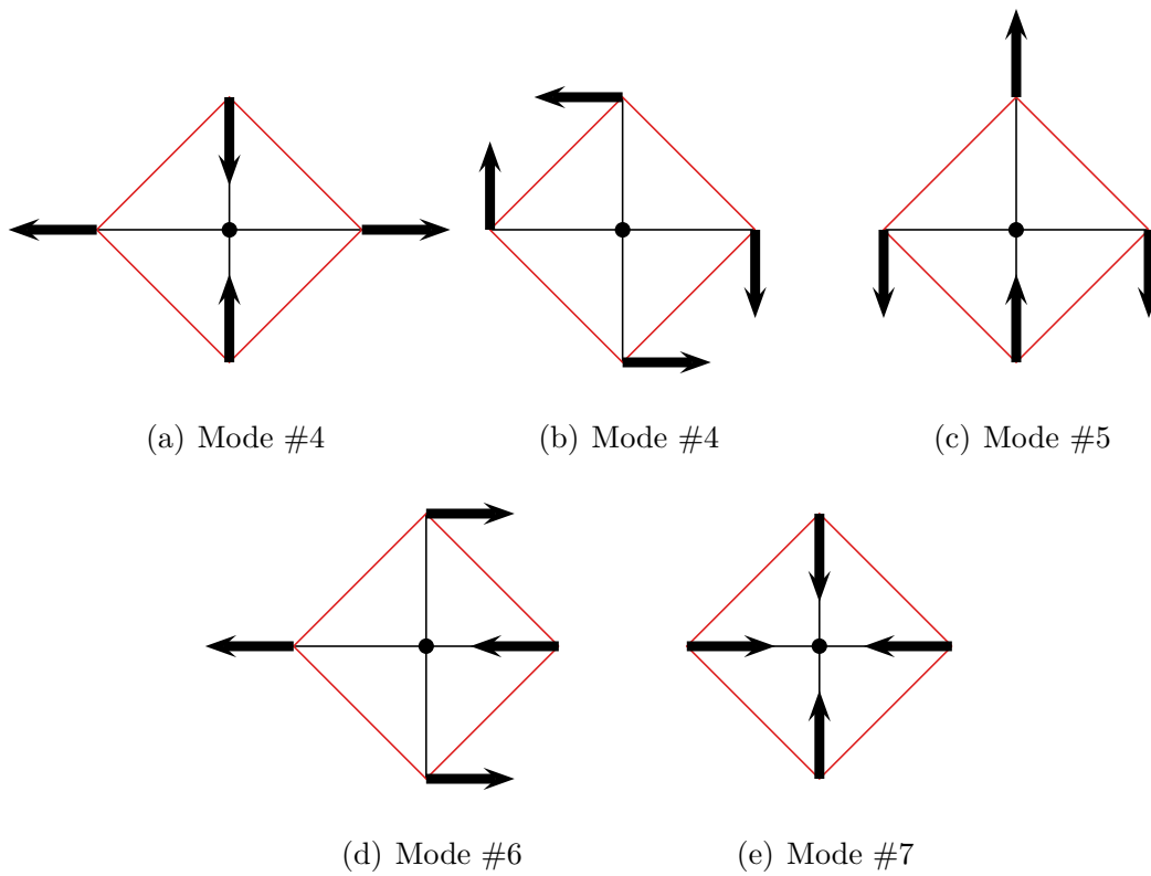
Figure 2.6: Planar tensegrity cross elastic modal vectors
