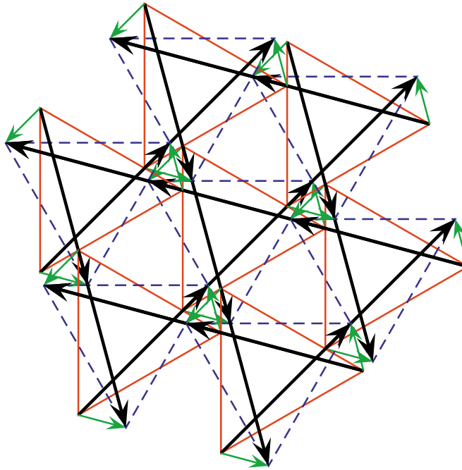
Figure 3.38: Three-bar plate – topology B – top view
