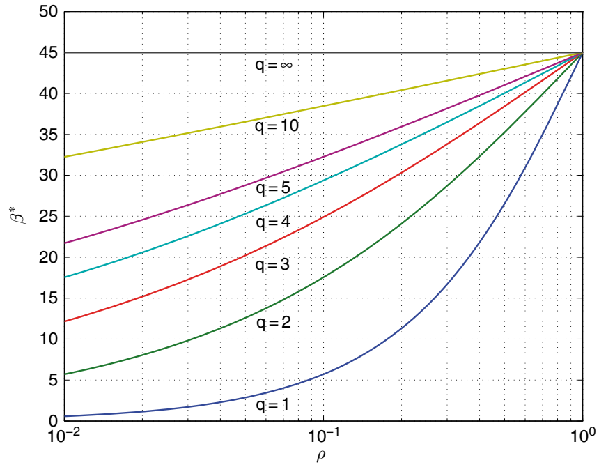
Figure 4.9: The optimal departure angle \beta^*
