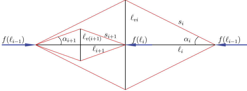
Figure 3.7: T-Bar self-similar iteration
