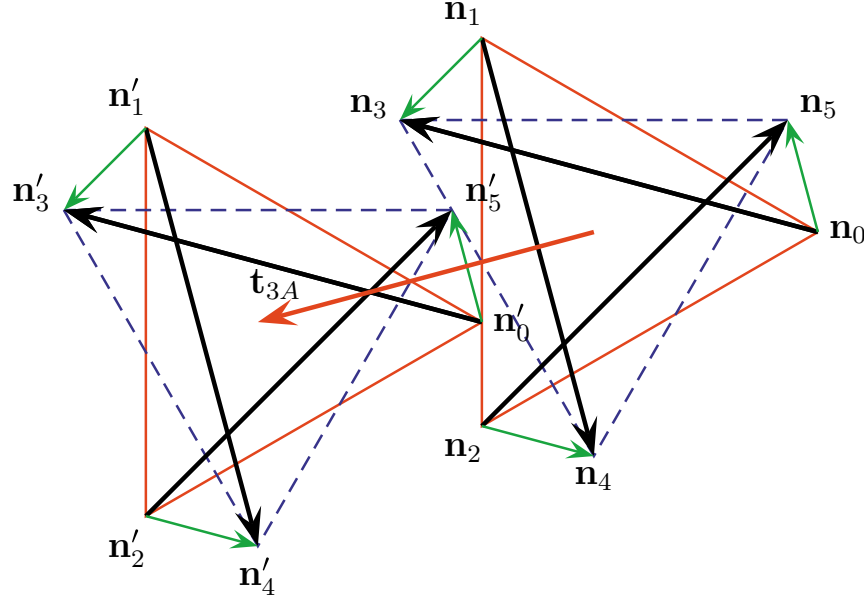
Figure 3.35: Three-bar plate connection – topology A – top view
