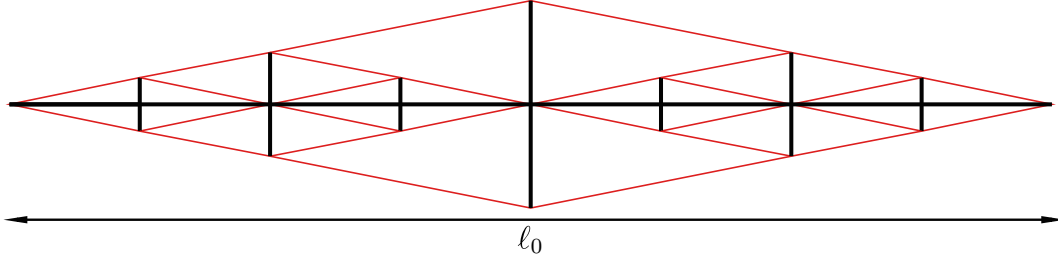
Figure 3.9: T-Bar self-similar n = 4 , constant \alpha
