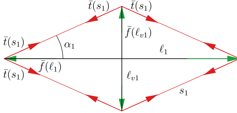
Figure 3.5: T-Bar forces for unloaded (prestressed) case, f(\ell_0) = 0
