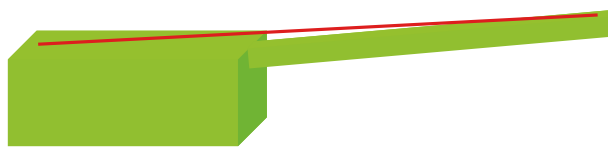
Figure 1.4: A single rigid body, a single string class 1 tensegrity system
