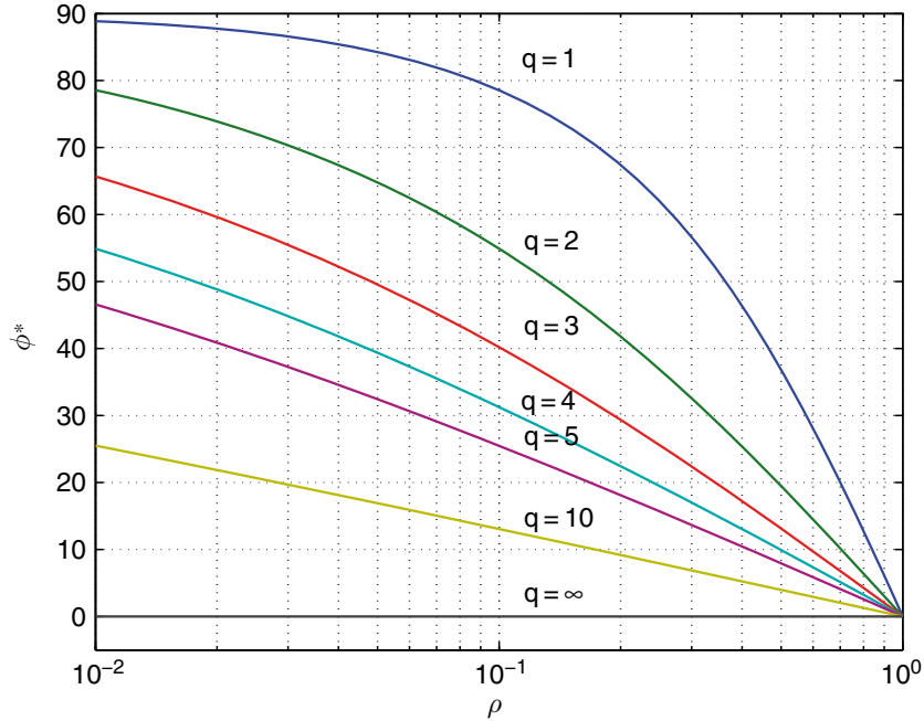
Figure 4.7: The optimal angle \phi^* (in degrees)
