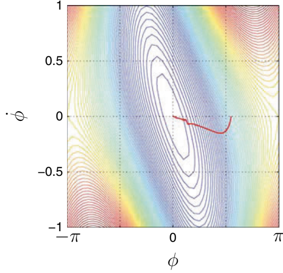
Figure 6.1: The Lyapunov landscape of V_\phi(\phi, \dot{\phi}) with system trajectory from Lyapunov-based control design with \delta = 0.20 and optimization of \|\mathbf{u}\|_2 . This Lyapunov function uses \alpha = \beta = 1 and \gamma = 3/2
