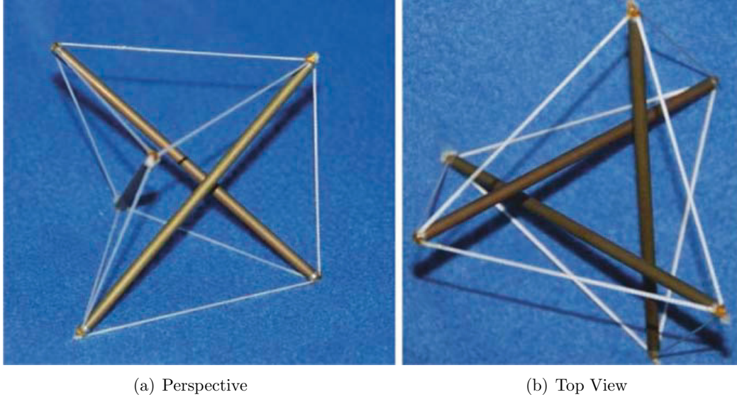
Figure 3.28: A regular minimal three-bar tensegrity prism
