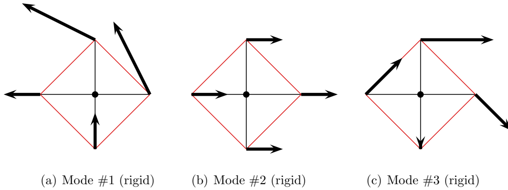
Figure 2.5: Planar tensegrity cross rigid modal vectors
