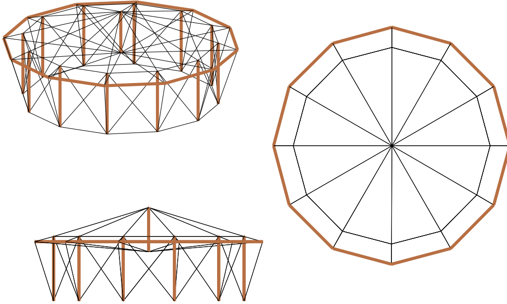
Figure 1.17: A class 2 tensegrity shelter
