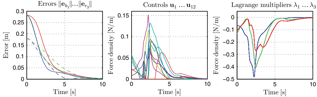
Figure 6.8: Data from simulation of the tensegrity prism with Lyapunov-based control design and optimization of \|\mathbf{u}\|_2 . For coordinates blue , green , and red denote x-, y-, and z-components, respectively. For the error norms we use blue , green , and red for errors related to rod 1, 2, and 3, respectively. That gives \|\mathbf{e}_{b_1}\| , \|\mathbf{e}_{b_2}\| , \|\mathbf{e}_{b_3}\| , \|\mathbf{e}_{r_1}\| , \|\mathbf{e}_{r_2}\| , \|\mathbf{e}_{r_3}\| . Further, Solid lines denote the errors \mathbf{b}_i , i = 1, 2 and 3 , while dashed lines denote the errors \mathbf{r}_i , i = 1, 2 and 3 . The color code for control inputs, and strings, are u_1 , u_2 , u_3 , u_4 , u_5 , u_6 , and u_7 . This combination is repeating for systems with more than seven inputs, such as this one
