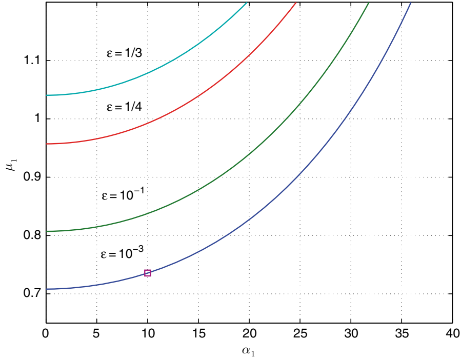
Figure 3.19: D-Bar unit: \mu_1 versus \alpha_1 , from (3.37)
