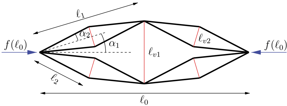
Figure 3.18: A D-Bar , n = 2 structure with \alpha_1 > \alpha_2
