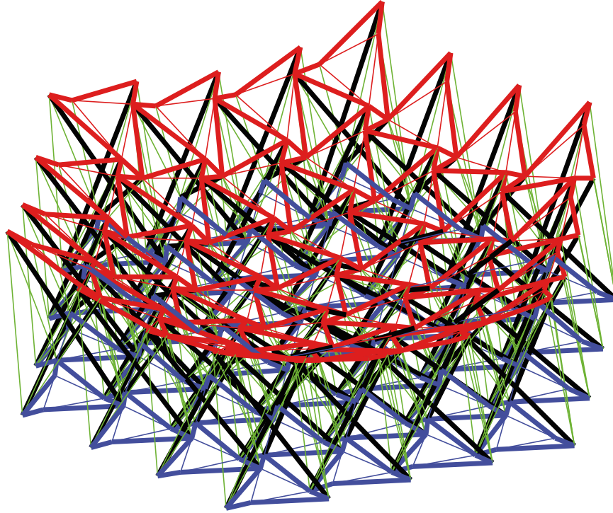
Figure 1.31: The same topology as the flat plate, but radii for top of each prism controlled to 90% of the radii of each prism in the bottom surface
