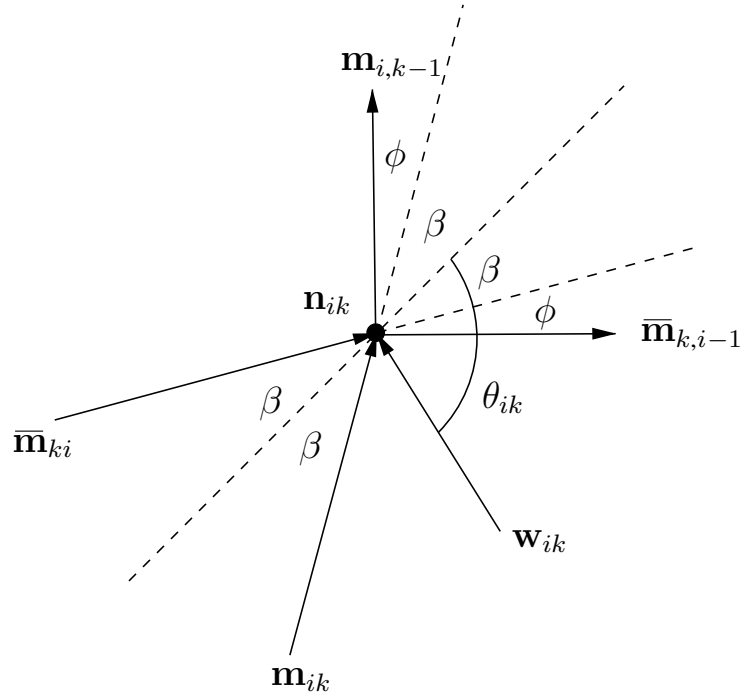
Figure 4.5: Sum of the forces at node \mathbf{n}_{ik}
