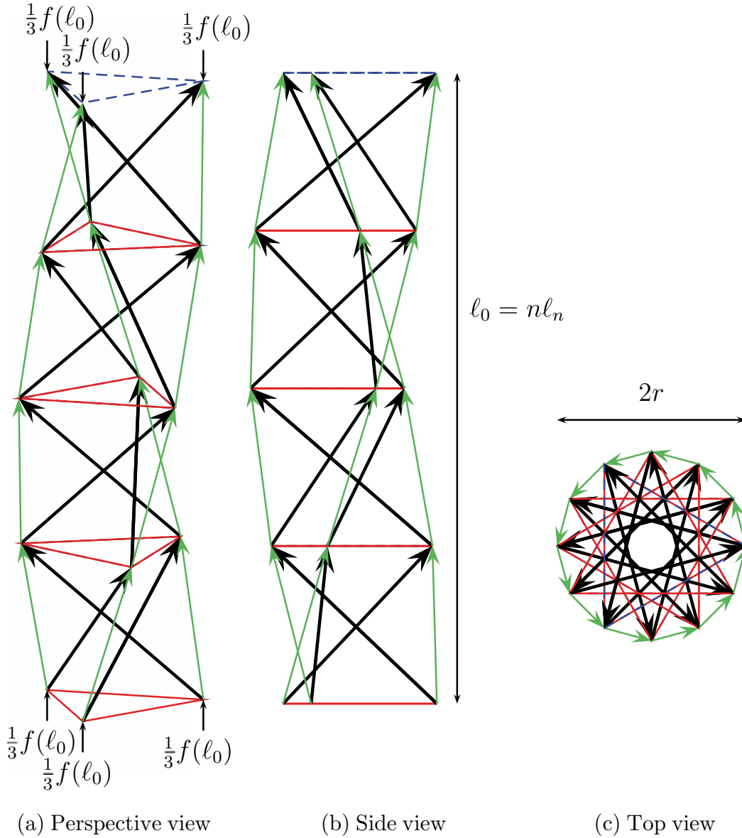
Figure 3.31: Unit-self-similar tensegrity column under compressive load
