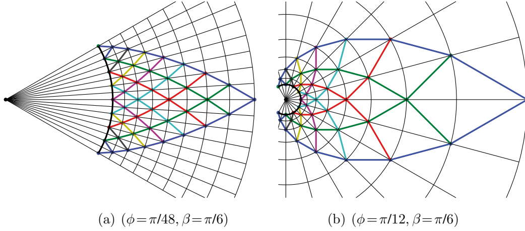
Figure 4.4: Michell Topologies of order 8
