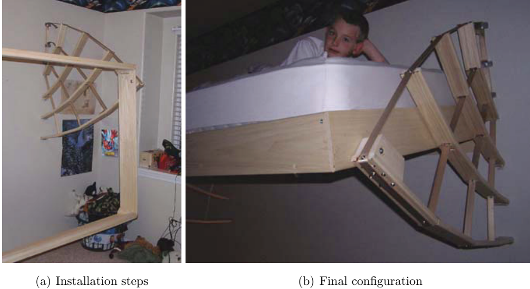
Figure 1.33: Wall-mounted bunk bed made from an optimal tensegrity configuration for bending loads
