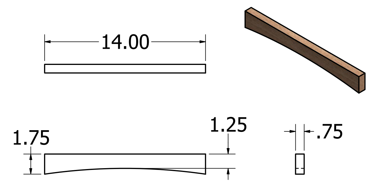
Rail - Front, Lower
