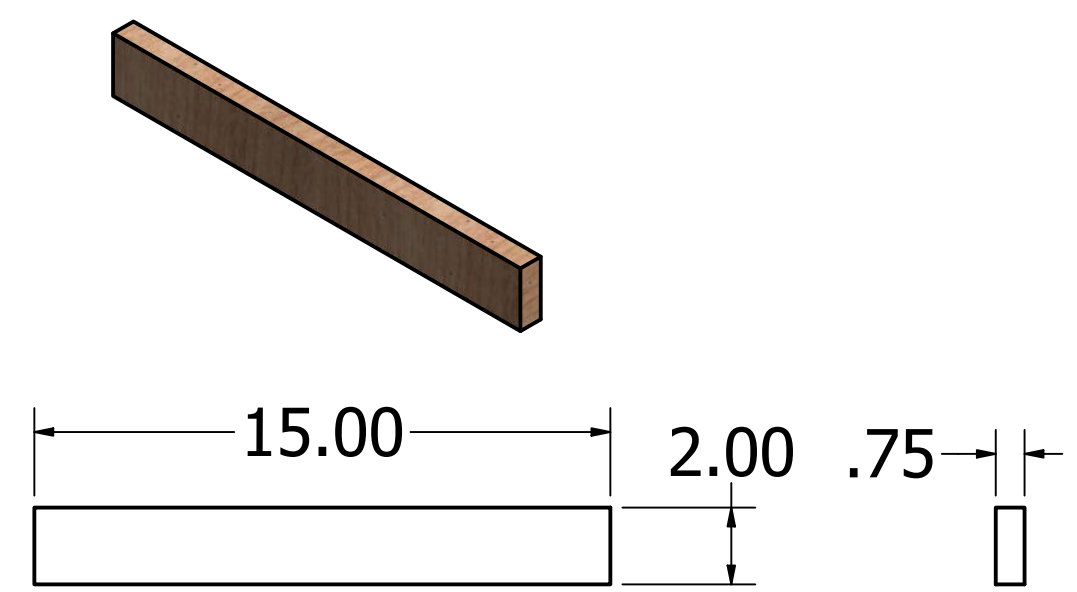
Slide Support (x4)
