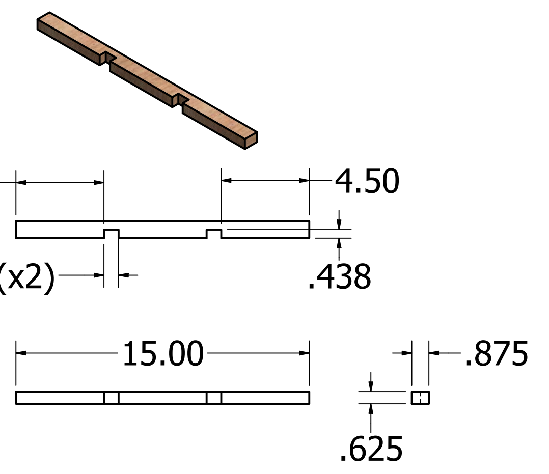
Support #3 (x2) (used on top)
