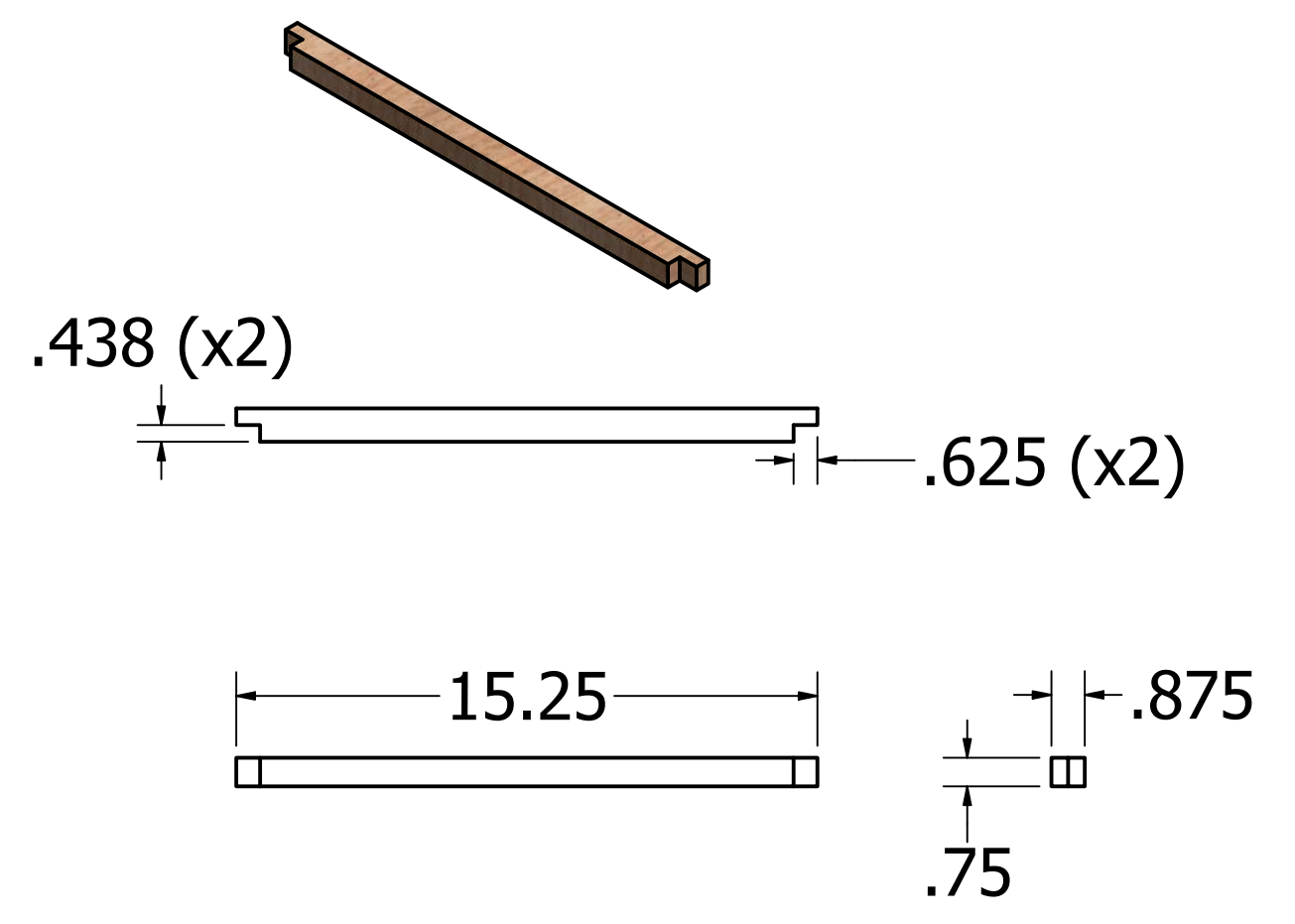
Support #4 (x2) (used to top)
