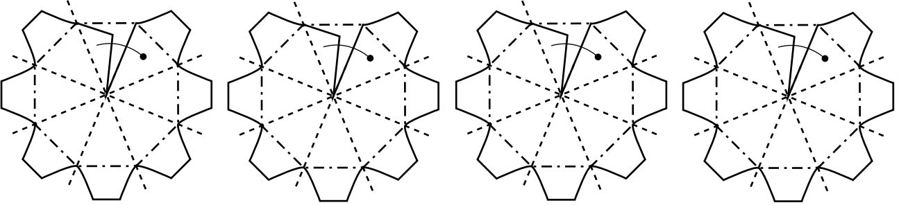
wheel mudguard
