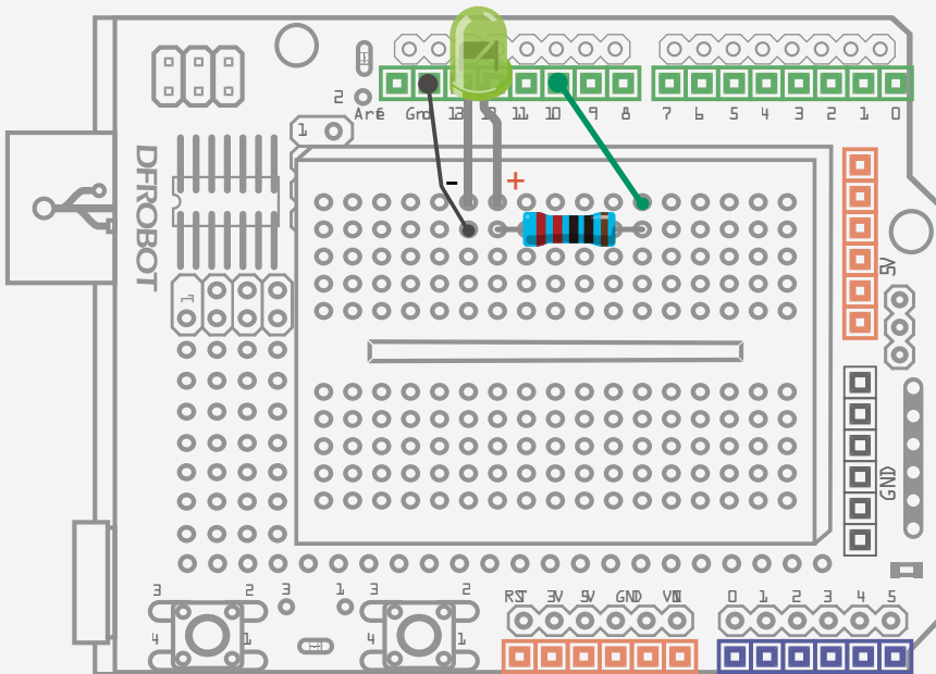
Fig. 4-1 Breathing LED Diagram
